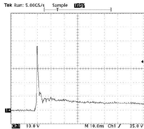
TLP Curve
